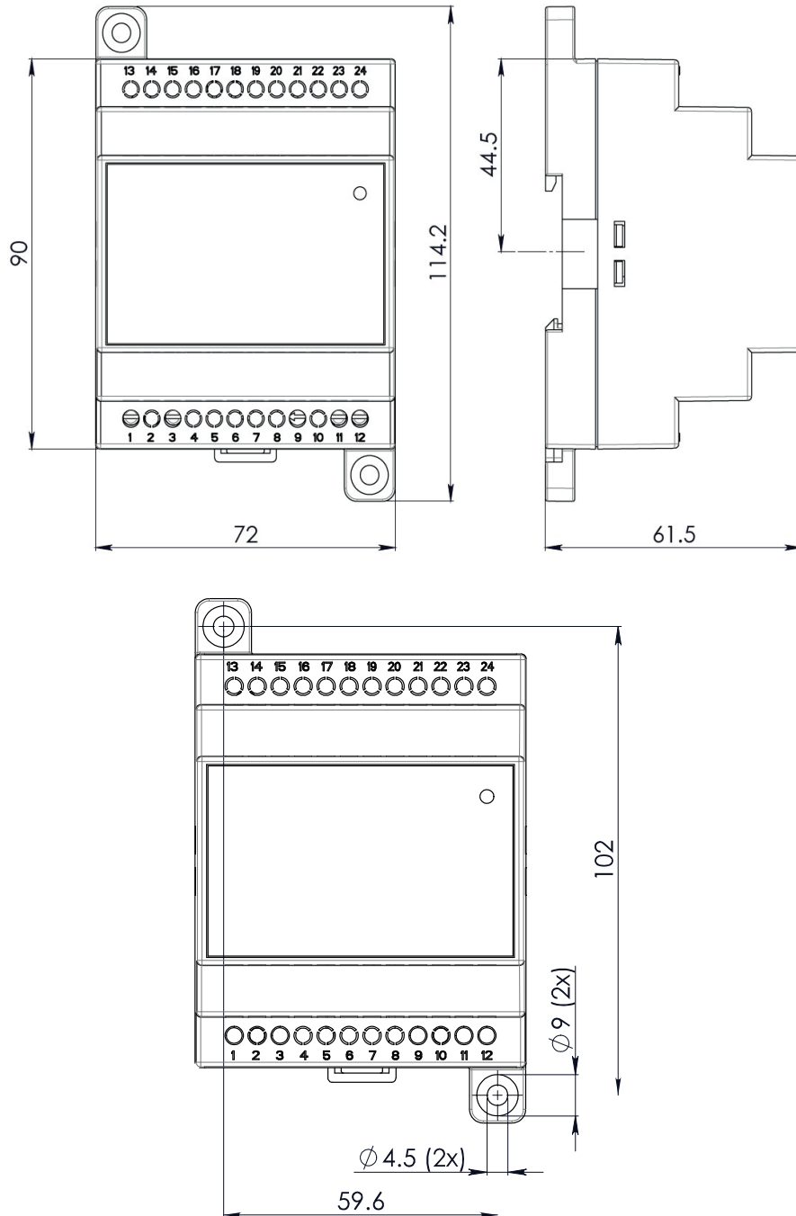
Figure 1. Mechanical Drawing
