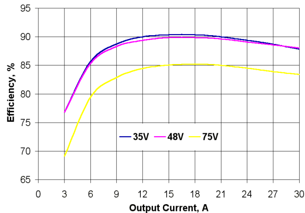
Figure 3. HLS30ZD (2.5V) Efficiency vs. Output Load
