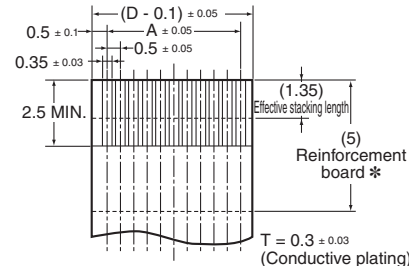
Recommended FPC Dimensions
