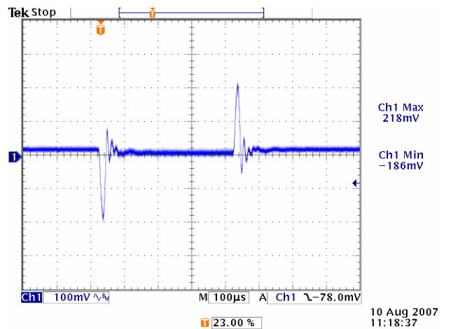
Figure 13. Vin=12V, Vout=2.5V
