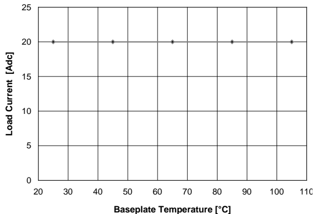
Figure 4. Coldplate cooling: Power derating of SQL48T20033-xxxBx converter with baseplate option and coldplate cooling. No thermal derating required. (Conditions: Air velocity \leq 30\text{LFM} ( \leq 0.15\text{m/s} ), V_{in} = 48\text{ V} , T_B \leq 105^\circ\text{C} )
