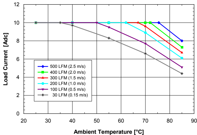
Fig. 5.0V.1: Available load current vs. ambient air temperature and airflow rates for SQ48T10050 converter with D height pins mounted vertically with V_{in} = 48\text{V} , air flowing from pin 3 to pin 1, and maximum FET temperature \leq 120^\circ\text{C} .
