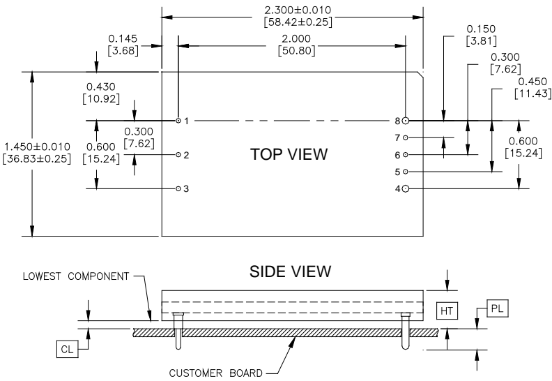
QM48T (Through-hole)
