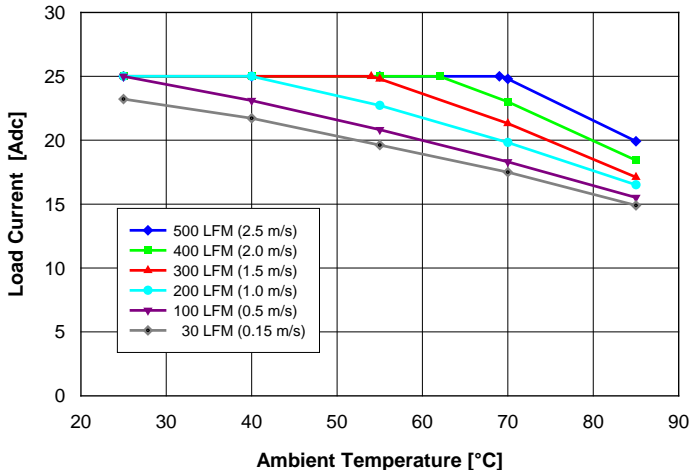
Fig. 1: Available load current vs. ambient air temperature and airflow rates for QM48T25050 converter with B height pins mounted vertically with air flowing from pin 3 to pin 1, MOSFET temperature \leq 120^{\circ}\text{C} , V_{in} = 48\text{ V} .
