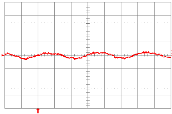
Fig. 14: Input reflected ripple current, i_s (10 mA/div), measured through 10 \mu H at the source at full rated load current and V_{in} = 48 V. Refer to Fig. 13 for test setup. Time scale: 1 \mu s/div.
