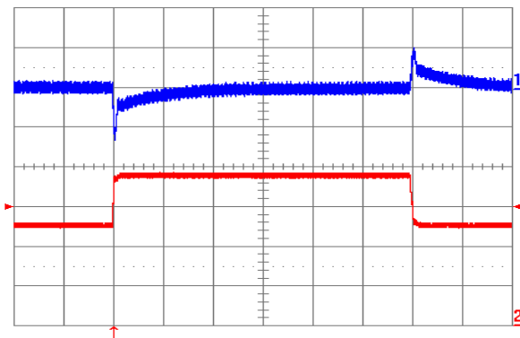
Fig. 11: Output voltage response to load current step-change (12.5 A – 18.75 A – 12.5 A) at V_{in} = 48\text{ V} . Top trace: output voltage (100 mV/div.). Bottom trace: load current (5 A/div.). Current slew rate: 1 A/ \mu\text{s} . C_o = 470\text{ }\mu\text{F} tantalum + 1 \mu\text{F} ceramic. Time scale: 0.2 ms/div.
