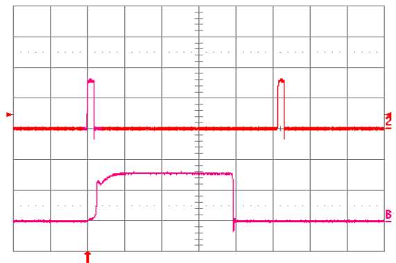
Fig. 17: Load current (top trace, 20 A/div, 20 ms/div) into a 10 m \Omega short circuit during restart, at V_{in} = 48 V. Bottom trace (20 A/div, 1 ms/div) is an expansion of the on-time portion of the top trace.
