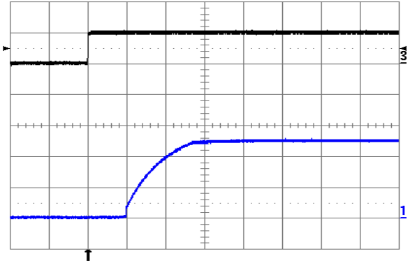
Fig. 10: Turn-on transient at full rated load current (resistive) plus 10,000 \mu\text{F} at V_{in} = 48\text{ V} , triggered via ON/OFF pin. Top trace: ON/OFF signal (5 V/div.). Bottom trace: output voltage (2 V/div.). Time scale: 2 ms/div.
