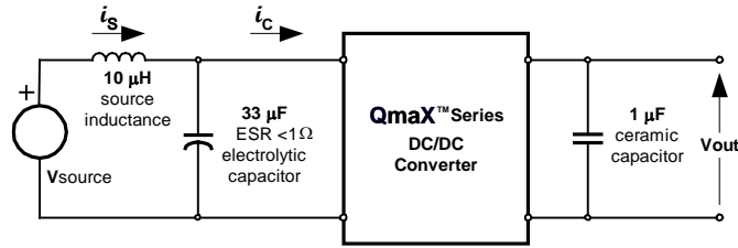
Fig. 13: Test setup for measuring input reflected ripple currents, i_c and i_s .
