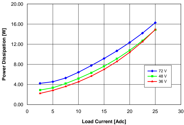
Fig. 7: Power dissipation vs. load current and input voltage for converter mounted vertically with air flowing from pin 3 to pin 1 at a rate of 300 LFM (1.5 m/s) and T_a = 25^\circ\text{C} .
