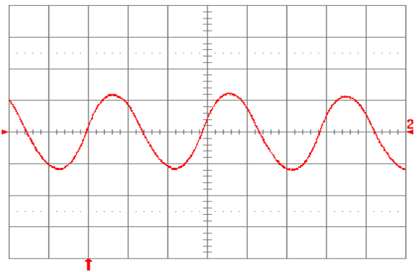
Fig. 15: Input reflected ripple current, i_c (200 mA/div), measured at input terminals at full rated load current and V_{in} = 48 V. Refer to Fig. 13 for test setup. Time scale: 1 \mu s/div.
