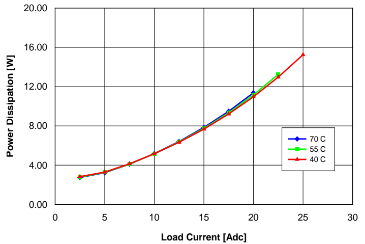
Fig. 8: Power dissipation vs. load current and ambient temperature for converter mounted vertically with V_{in} = 48\text{ V} and air flowing from pin 3 to pin 1 at a rate of 200 LFM (1.0 m/s).
