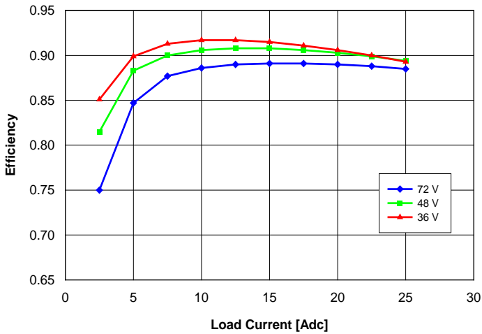
Fig. 5: Efficiency vs. load current and input voltage for converter mounted vertically with air flowing from pin 3 to pin 1 at a rate of 300 LFM (1.5 m/s) and T_a = 25^\circ\text{C} .
