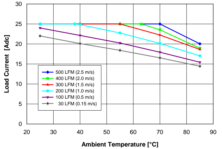
Fig. 2: Available load current vs. ambient air temperature and airflow rates for QM48T25050 converter with B height pins mounted horizontally with air flowing from pin 3 to pin 1, MOSFET temperature \leq 120^{\circ}\text{C} , V_{in} = 48\text{ V} .
