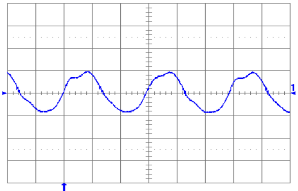
Fig. 12: Output voltage ripple (20 mV/div.) at full rated load current into a resistive load with C_o = 10\text{ }\mu\text{F} tantalum + 1 \mu\text{F} ceramic and V_{in} = 48\text{ V} . Time scale: 1 \mu\text{s} /div.
