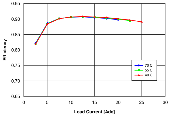
Fig. 6: Efficiency vs. load current and ambient temperature for converter mounted vertically with V_{in} = 48\text{ V} and air flowing from pin 3 to pin 1 at a rate of 200 LFM (1.0 m/s).
