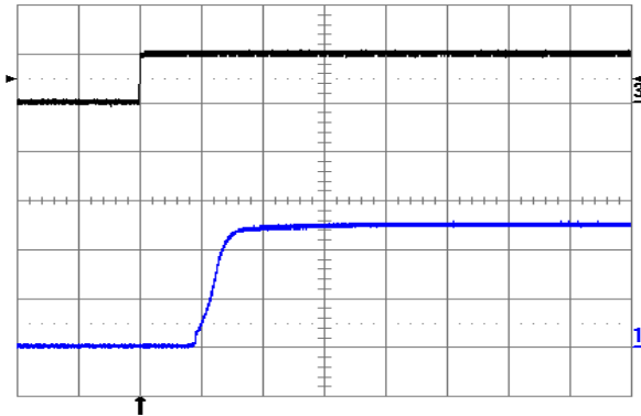
Fig. 9: Turn-on transient at full rated load current (resistive) with no output capacitor at V_{in} = 48\text{ V} , triggered via ON/OFF pin. Top trace: ON/OFF signal (5 V/div.). Bottom trace: output voltage (2 V/div.) Time scale: 2 ms/div.
