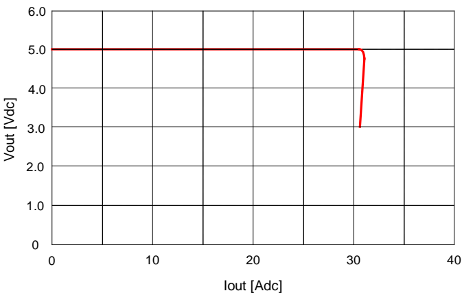
Fig. 16: Output voltage vs. load current showing current limit point and converter shutdown point. Input voltage has almost no effect on current limit characteristic.
