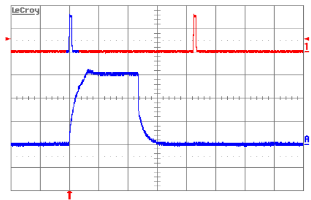
Figure 13. Input reflected ripple-current, i_C (200 mA/div.), measured at input terminals at full rated load current and V_{in} = 48 \text{ V} . Refer to Error! Reference source not found. for test setup. Time scale: 1 \mu\text{s}/\text{div} .
