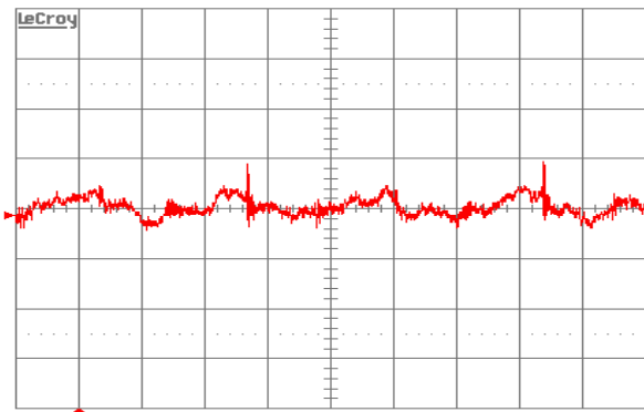
Figure 12. Input reflected-ripple current, i_S (10 mA/div.), measured through 10 \mu\text{H} at the source at full rated load current and V_{in} = 48 \text{ V} . Refer to Error! Reference source not found. for test setup. Time scale: 1 \mu\text{s}/\text{div} .
