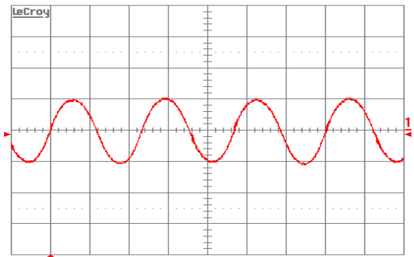
Figure 13. Input reflected ripple-current, i_C (200 mA/div.), measured at input terminals at full rated load current and V_{in} = 48 \text{ V} . Refer to Error! Reference source not found. for test setup. Time scale: 1 \mu\text{s}/\text{div} .
