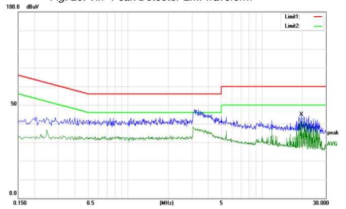
Fig. 20: Vin- Peak Detector EMI waveform
